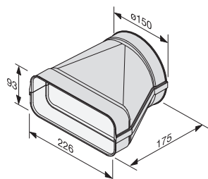
Adapter DFK-A
